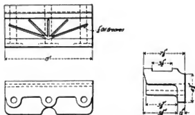
Figs. 1548-1550. Firebox Bearer for Consolidation (2-8-0) Locomotive.
